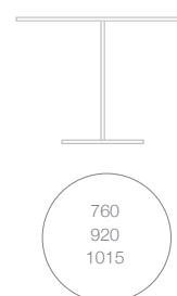
Dining Table - Pedestal h 760
