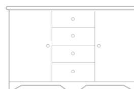
2 Door, 4 Drawer Sideboard h 790 w 1200 d 475
